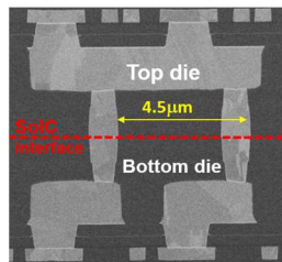
Fig.12 N2 optimizes pTSV and sTSV for F2F/F2B stacking w/ SoIC bond pitch →4.5 µm
